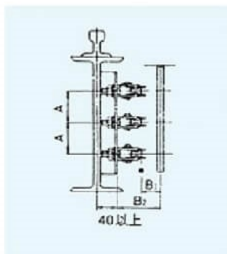
• 側式施工法 (On Side)
