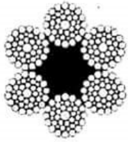
6xWS(41)FC
