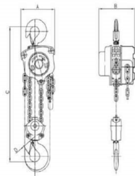
KT-C Chain Block (Double Chain)
