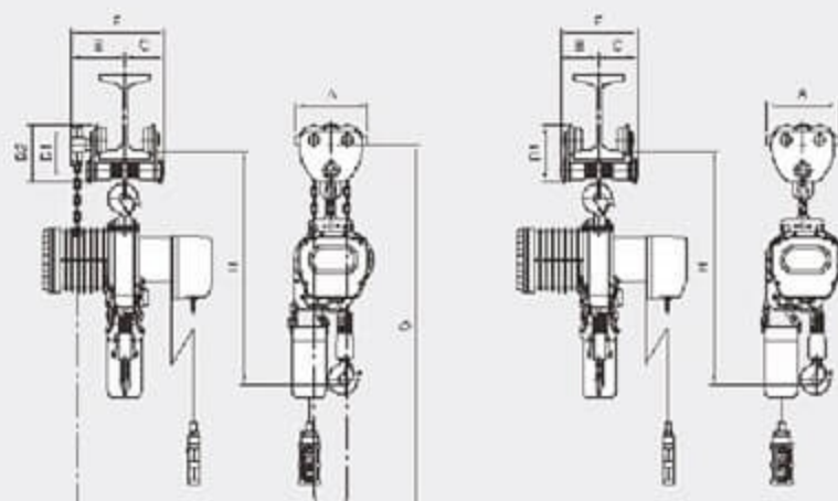
Hoist With GT
