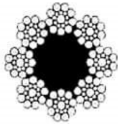
8xS(19)FC
