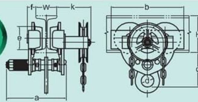
AGD Geared Trolley (Drop Stop)
