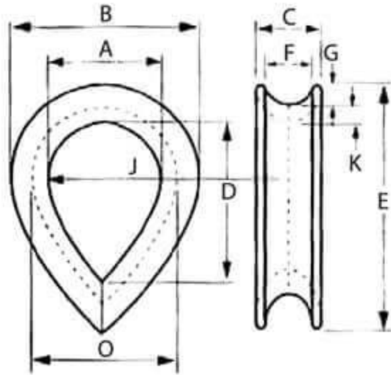
Ordinary Thimbles
