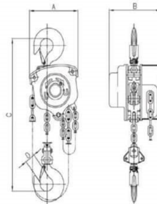
KT-C Chain Block (Single Chain)
