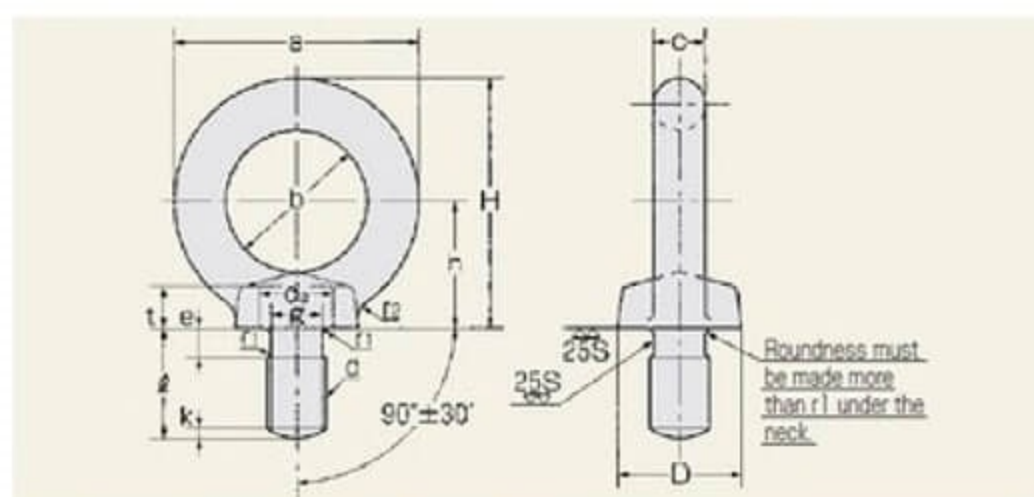
■Size Table of Eye Bolt
