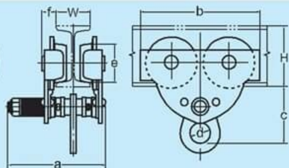
APD Plain Trolley (Drop Stop)
