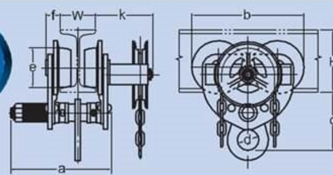
AG Geared Trolley
