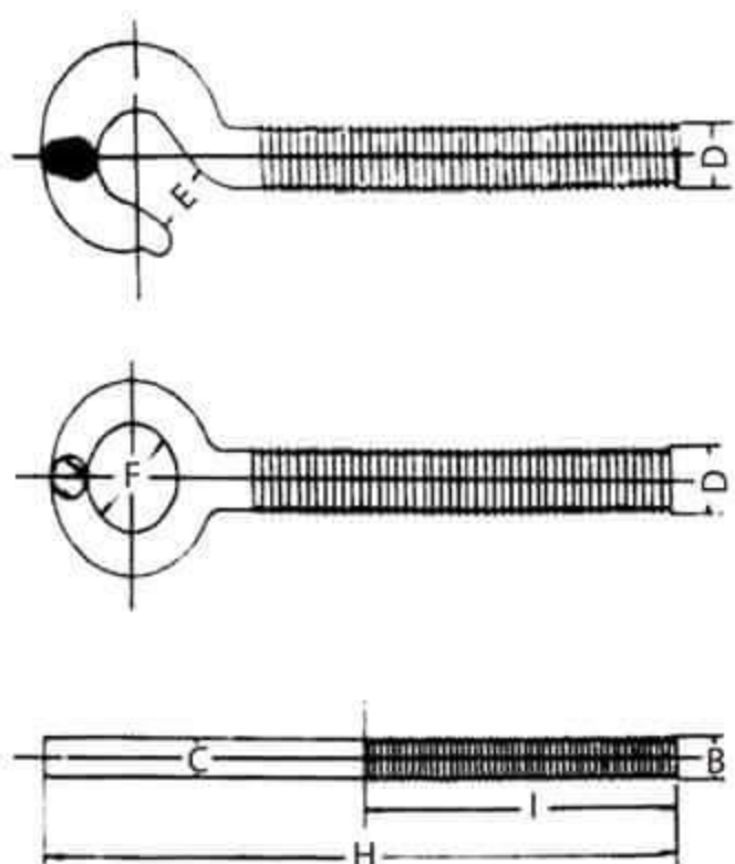
(7) Sizes and Weights (Approx.)
