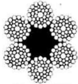
6xWS(41)FC
