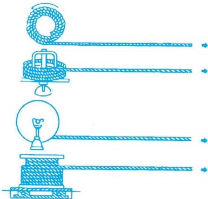
Correct Way
