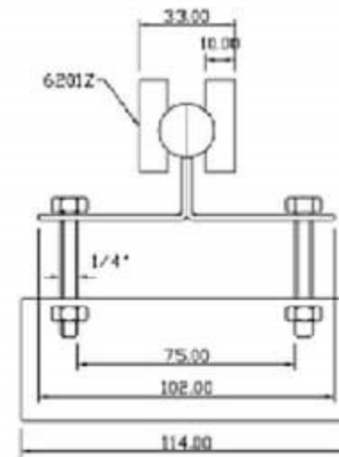
KY-BC4533 C40滑輪 Cable Trolley KY-BCS4533白鐵
