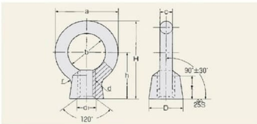
■Size Table of Eye Nut
