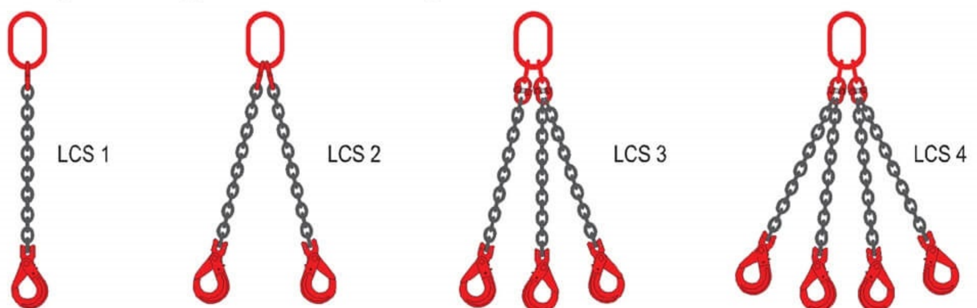
Chain sling 1, 2, 3, 4 legged with Clevis self locking hook
