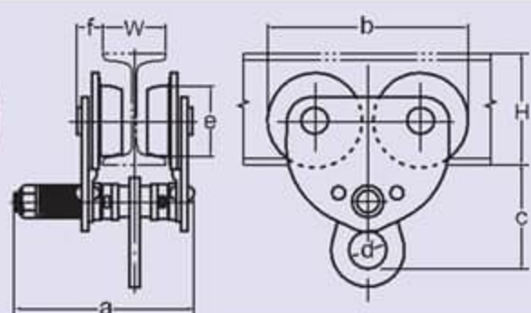
AP Plain Trolley
