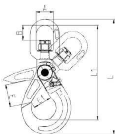
SLR-755 G80 EUROPEAN TYPE SWIVEL SELF-LOCKING HOOK
